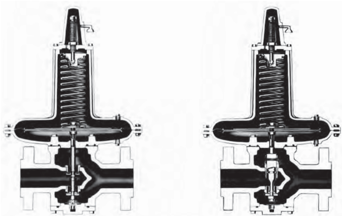
461-S with Double Seat Balanced Valve
